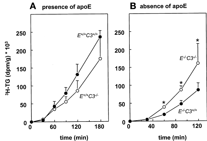
Fig. 3. Intestinal lipid absorption in wild-type and apoC3 knockout mice in the presence (A) and absence (B) of apoE. (A) Wild-type (solid circles) and apoC3 -/- (open circles) mice, and (B) apoE -/- (solid circles) and apoE -/- apoC3 -/- (open circles) mice were fasted overnight and received an intravenous injection of Triton WR1339. Subsequently, at time point 0 mice were administered an intragastric fat load (400 \mu\text{l} of olive oil) containing [ 3 H]TG. The appearance of 3 H label in the plasma TG fraction was measured over time as described in Materials and Methods. Values are depicted as means \pm SD of six mice per group. Note the difference in scale of the x axis of (A) and (B). * P < 0.05 .
